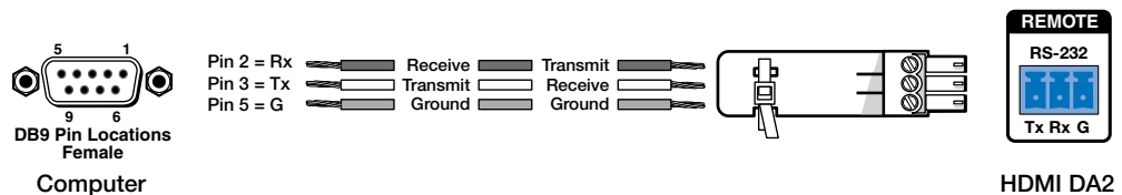
Figure 3. Wiring the HDMI DA2 for RS-232 Control
